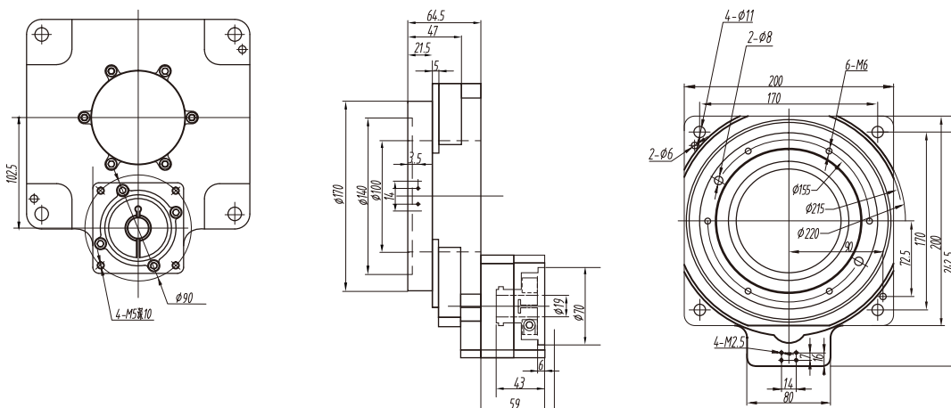
SH200-10-S(尺寸圖)
